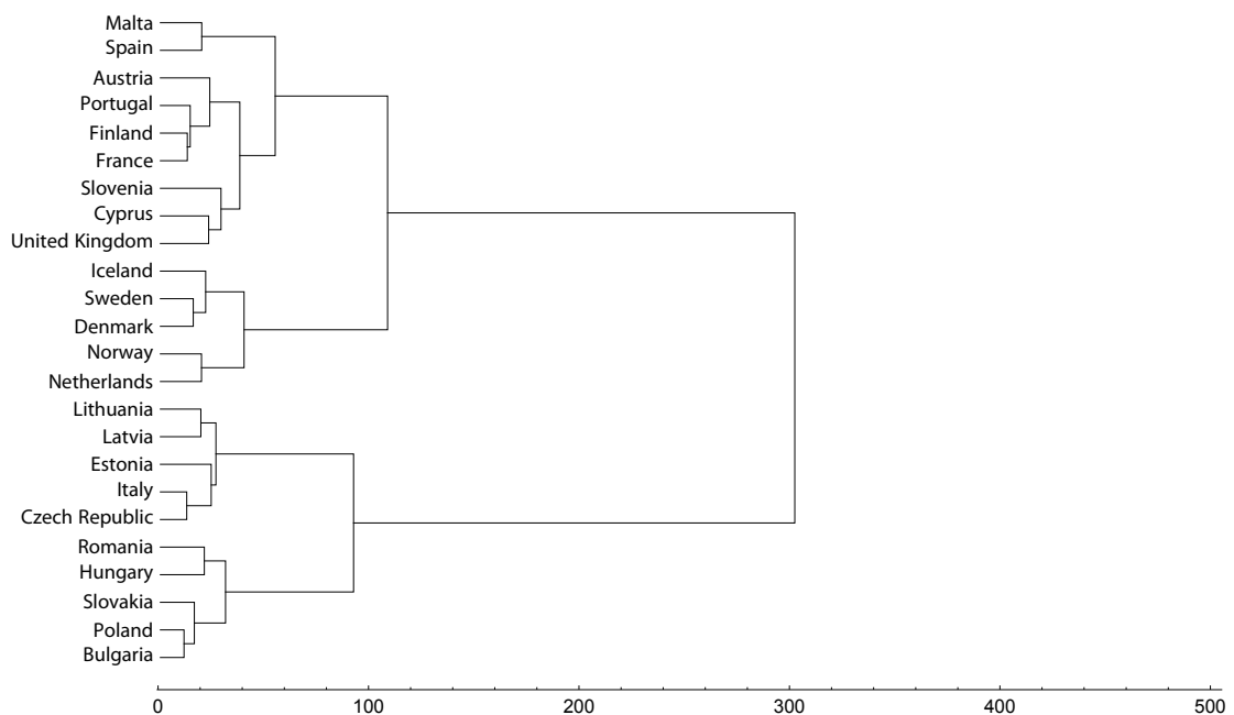
Fig. 3. Grouping countries by Ward's method—dendrogram for year 2013
